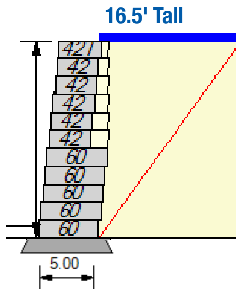
Use the LB42 and LB60 units for unreinforced walls up to 16.5'
