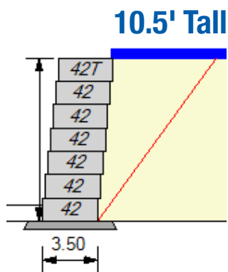
The LB42 units can build an unreinforced wall up to 10.5'
