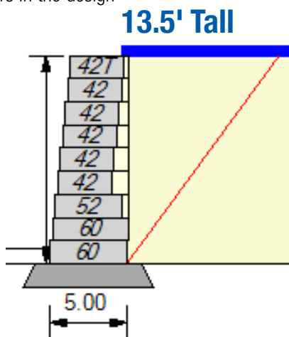
With LB42, LB52 and LB60 units reach heights up to 13.5'
